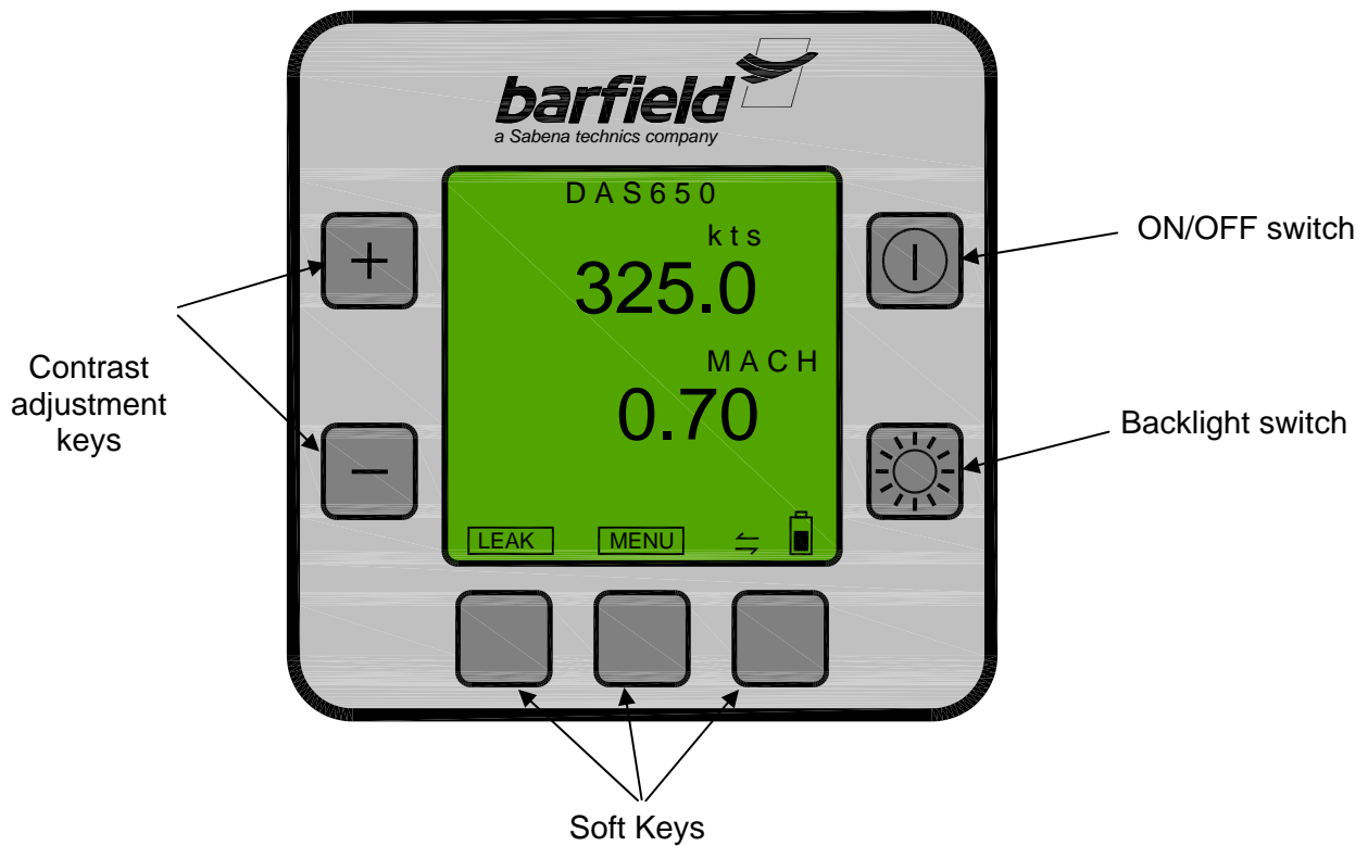
FIGURE 1 FUNCTION KEYS AND SOFT KEYS
